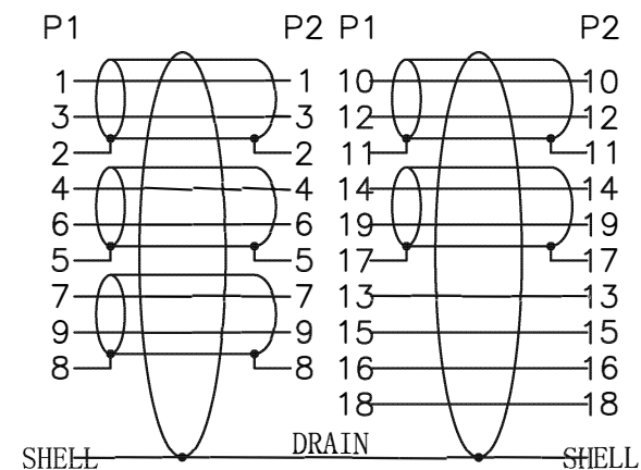
Pin Assignment
