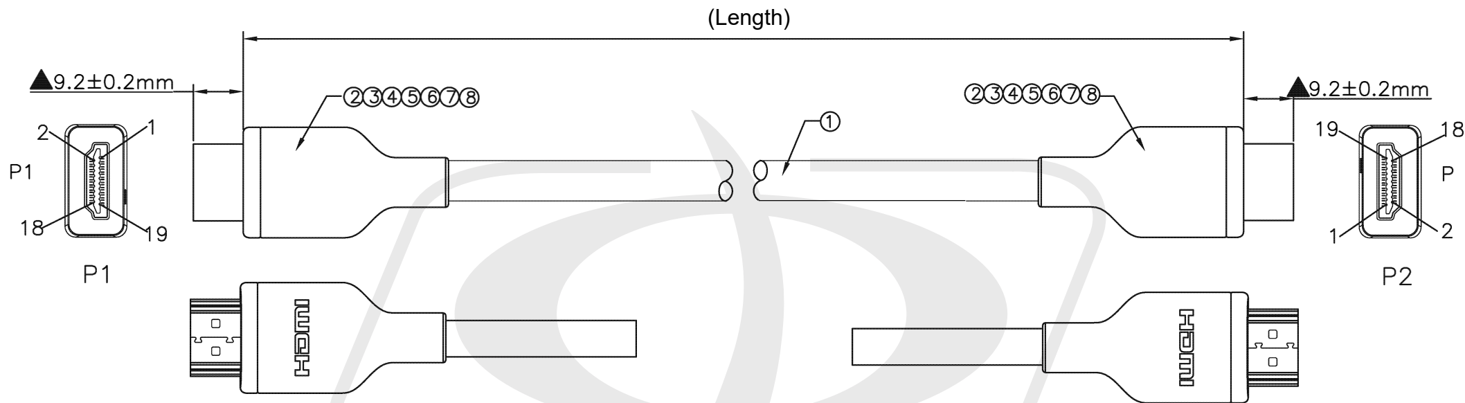
Pin Assignment
